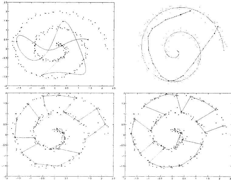
Fig. 1. A spiral with some noise. Results for (left to right, top to bottom): GTM, PLA, GCS and SOM.
