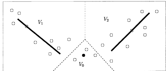
Fig. 2. An example where the data (open dots) are partitioned in three Voronoi regions for two normal segments ( V_1 and V_2 ) and one ( V_0 ) ‘zero-length’ segment (black dot).
