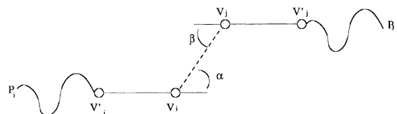
Fig. 3. Connecting two sub-paths: the angle penalty of (v_i, v_j) is the sum of the angles between an edge and the adjacent edges, i.e. \alpha + \beta .
