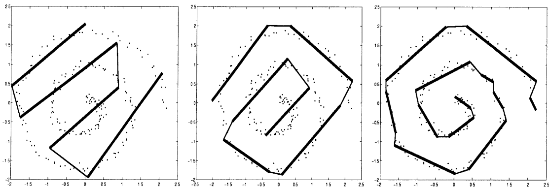
Fig. 6. Some of the PLs encountered (using 4, 6 and 12 segments, respectively), by the algorithm when fitting data distributed along a spiral.
