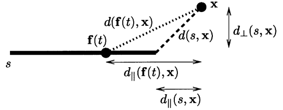
Fig. 4. Illustration of the distances between a point \mathbf{x} a segment s and a point \mathbf{f}(t) on s .
