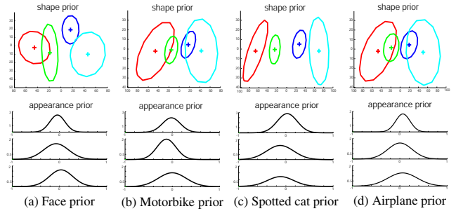
Figure 3: Prior distribution for shape mean ( \mu^{\mathcal{X}} ) and appearance mean ( \mu^{\mathcal{A}} ) for faces, motorbikes, spotted cats and airplanes. Each prior's hyperparameters are estimated from models learnt with maximum likelihood methods, using "the other" datasets [10]. For example, face prior is obtained from models of motorbikes, spotted cats and airplanes. Only the first three PCA dimensions of the appearance priors are displayed. All four parts of the appearance begin with the same prior distribution for each PCA dimension.
