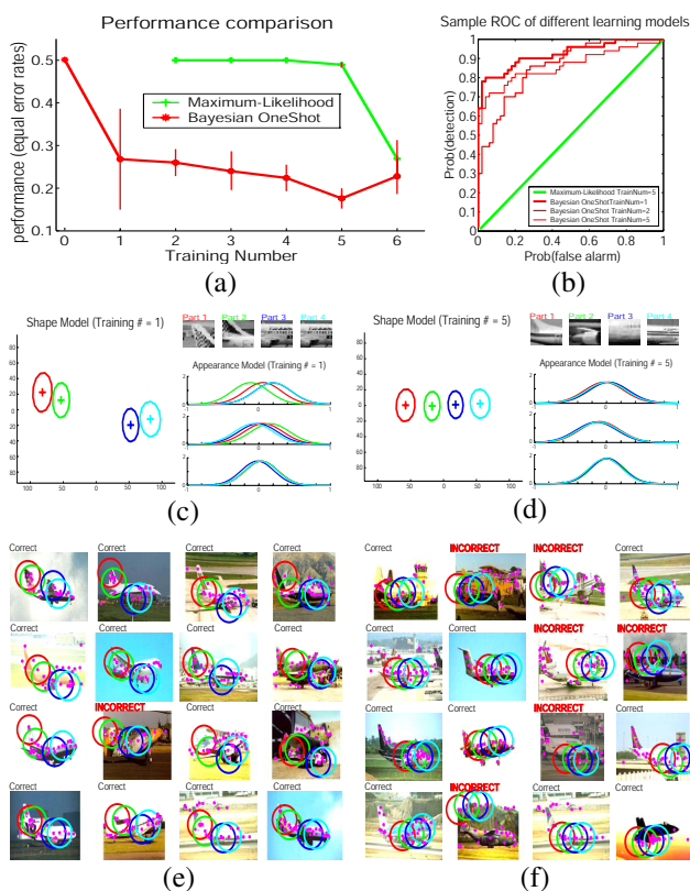
Figure 7: Summary of airplane model.
