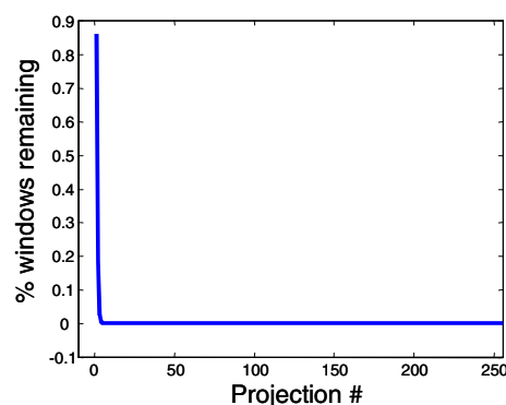
Figure 7: Percentage of image windows remaining after each projection for images of size 256 \times 256 and patterns of size 16 \times 16 . Results are averaged over 100 image-pattern pairs.
