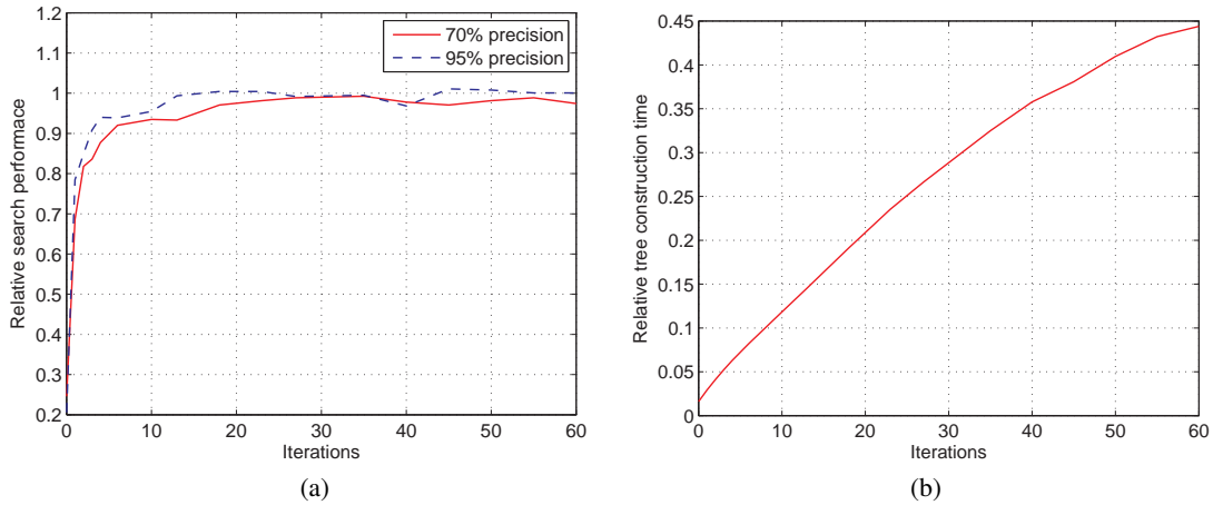
Figure 3: The influence that the number of k-means iterations has on the search time efficiency of the k-means tree (a) and on the tree construction time (b) (100K SIFT features dataset)
