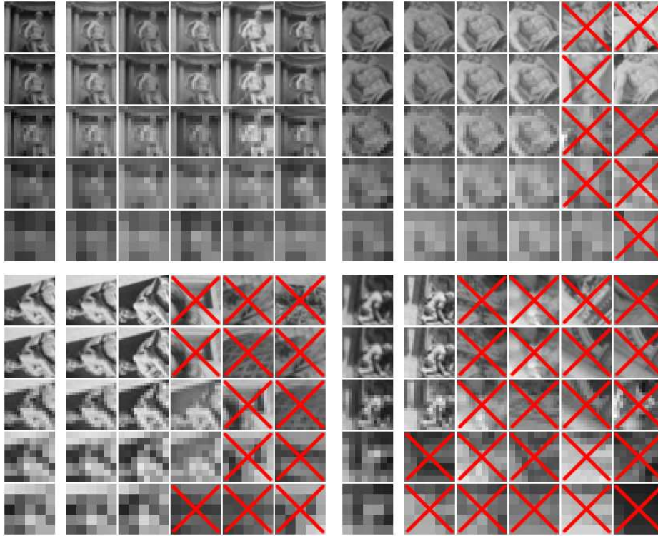
Figure 5: Examples of querying the Trevi Fountain patch dataset using different patch sizes. The query patch is on the left of each panel, while the following 5 patches are the nearest neighbors from a set of 100,000 patches. Incorrect matches are shown with an X.
